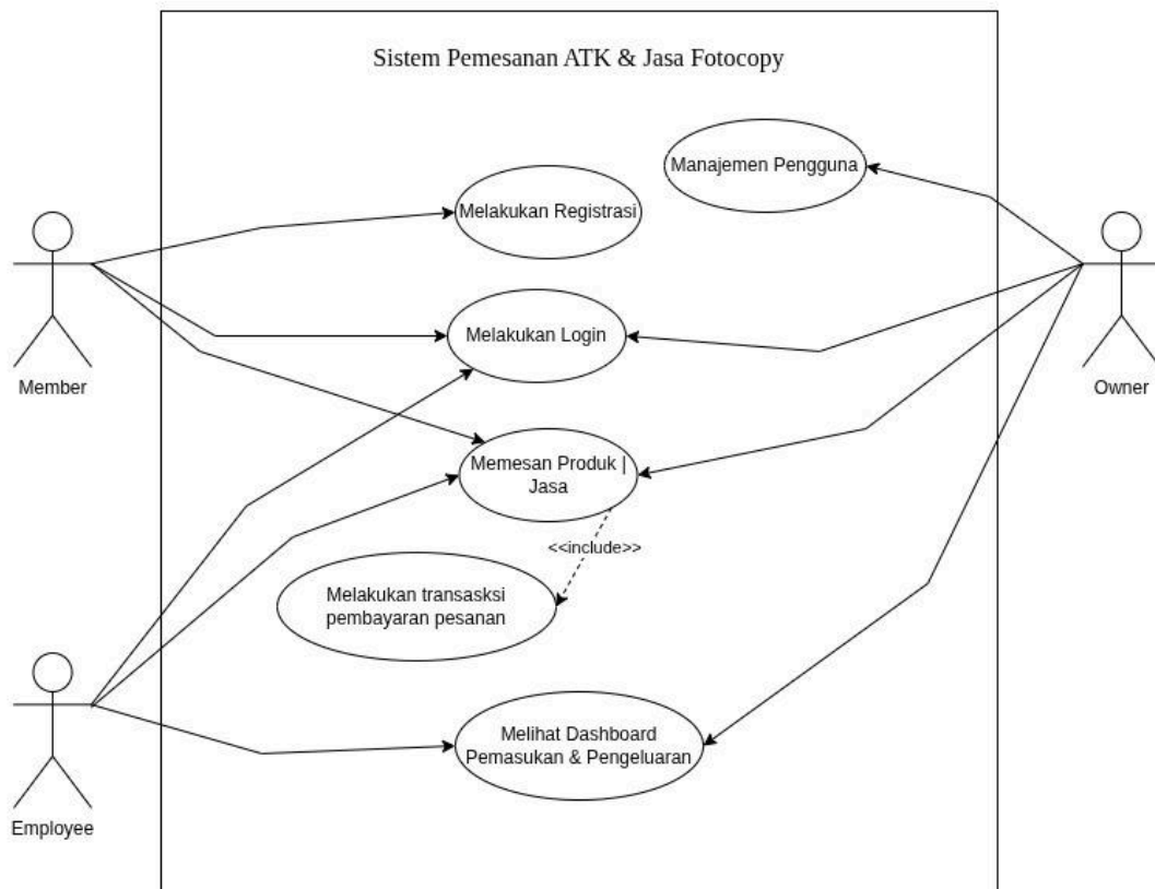
Gambar 5 Usecase Diagram
